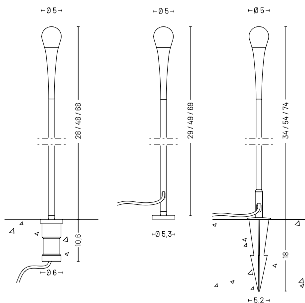
Mounting by housing box
